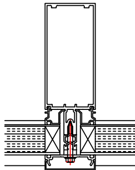
TYPICAL DETAIL FOR PANELS USED WITH CURTAIN WALLING SYSTEMS
