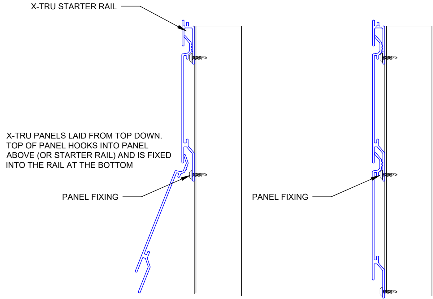
UNITY X-TRU INSTALLATION DETAIL
