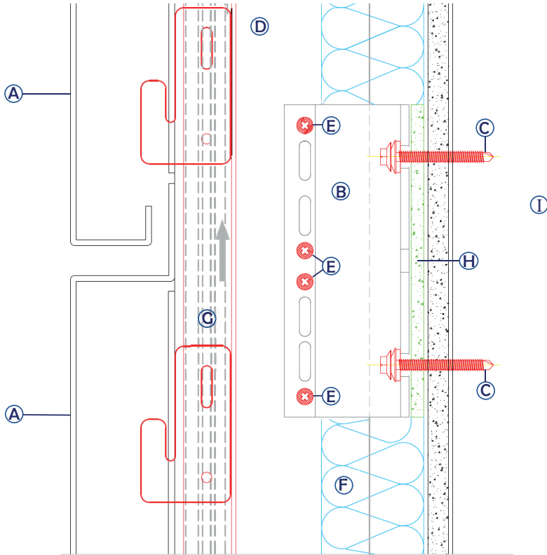
Vertical Section
