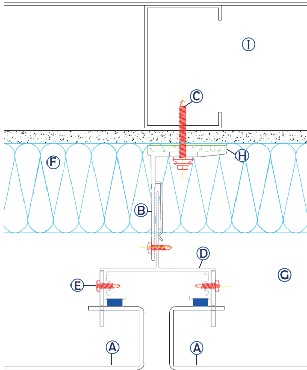
Horizontal Section
