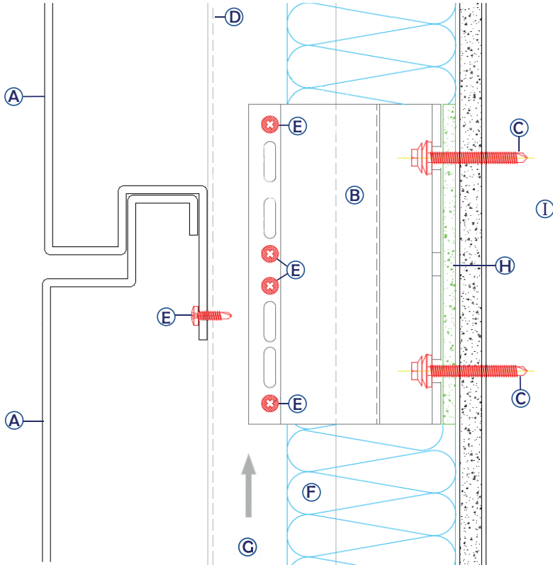
Vertical Section
