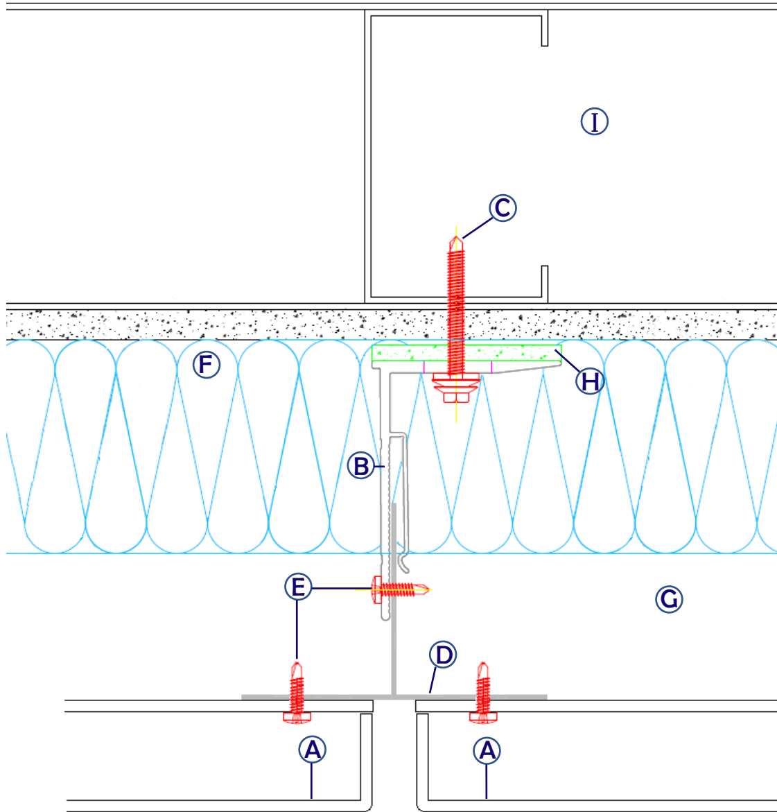
Plan View Joint Detail
