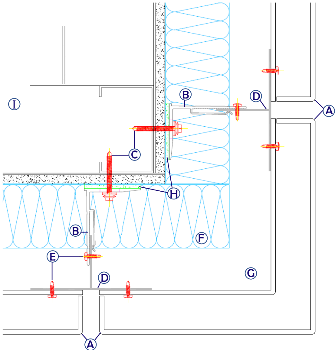
Plan View Corner Detail
