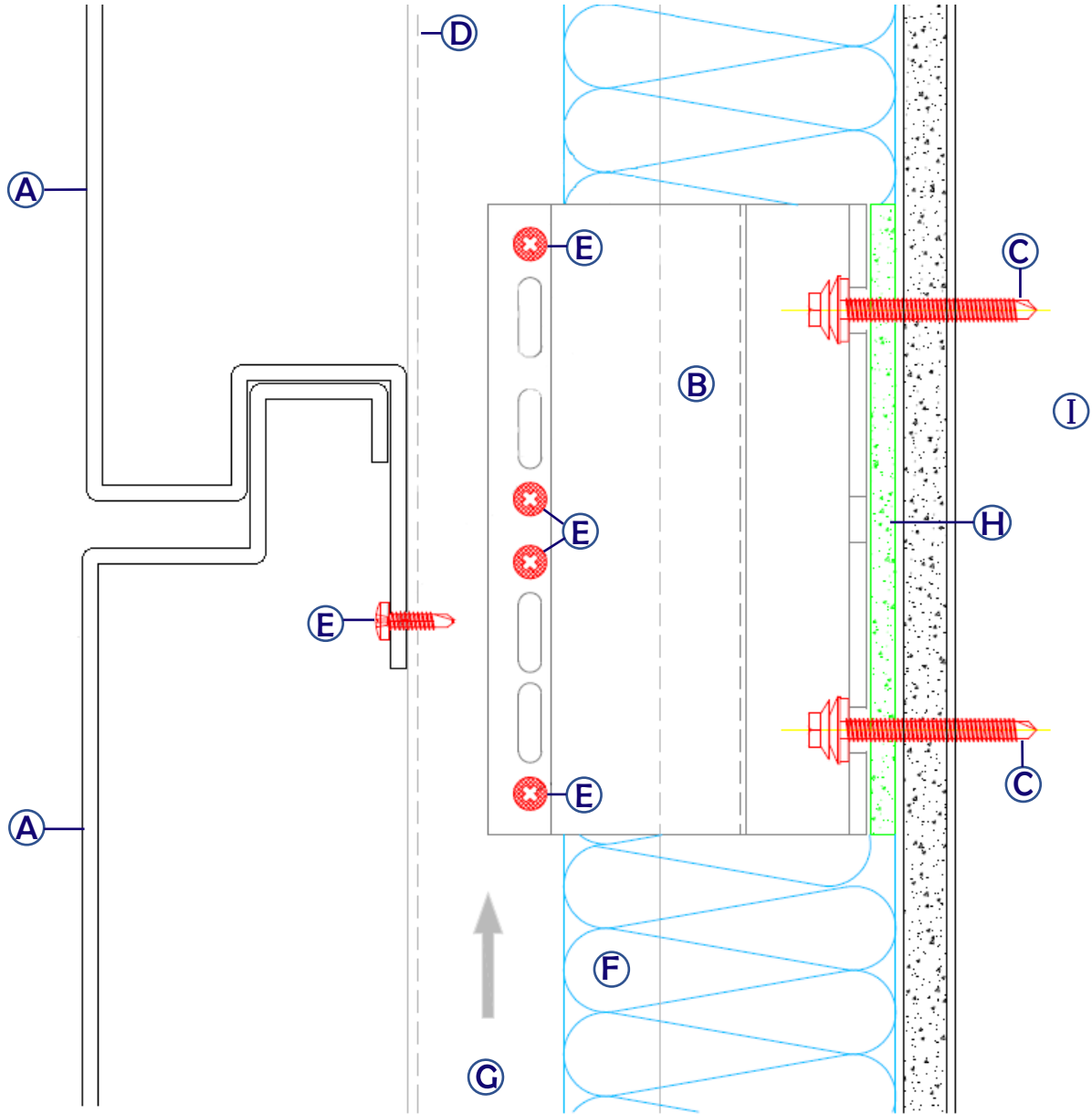
Side View Joint Detail
